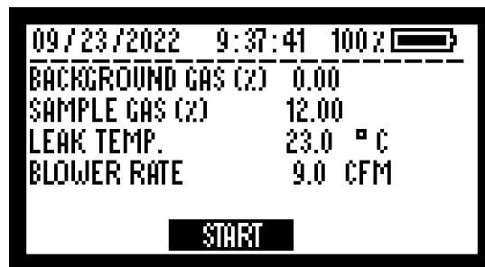
Figure 8. Selector on START
